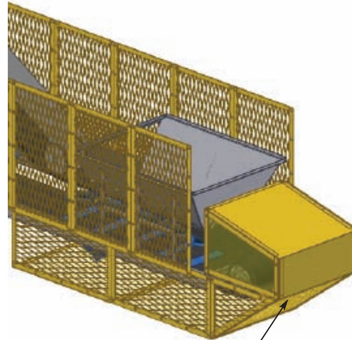
Tail section guarding utilizing standard Flat Guards and custom tail pulley enclosure. (See Pg 15 for Dimensional Data Requirements)
