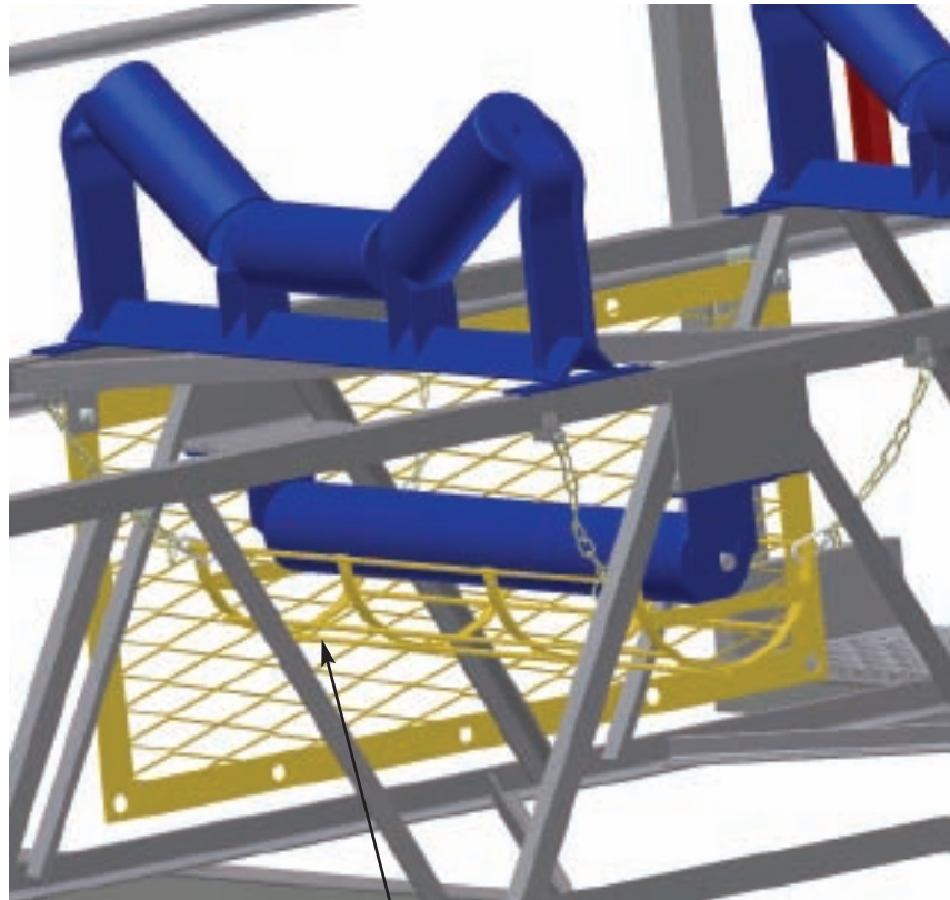
Standard Return Roller Basket with mounting kit.
